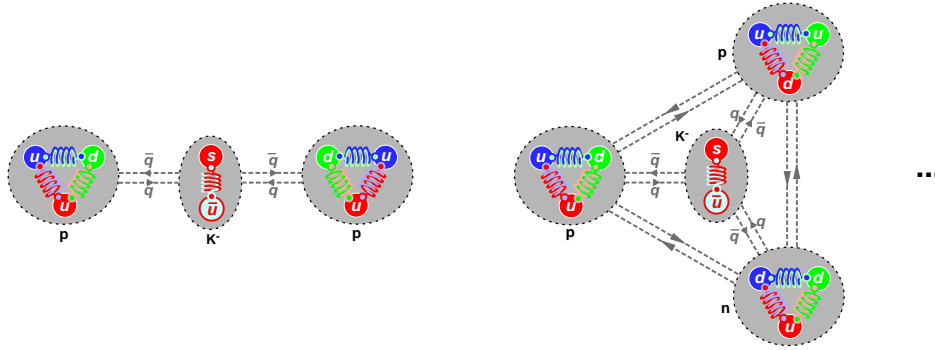
Figure 2: Schematic diagrams of possible kaonic bound states.
