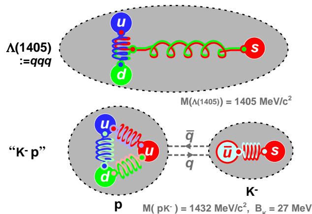
Figure 1: Schematic diagram of \Lambda(1405) as for baryon: qqq (top) and that of nucleon- \bar{K} bound state: “ K^-p ” (bottom).
