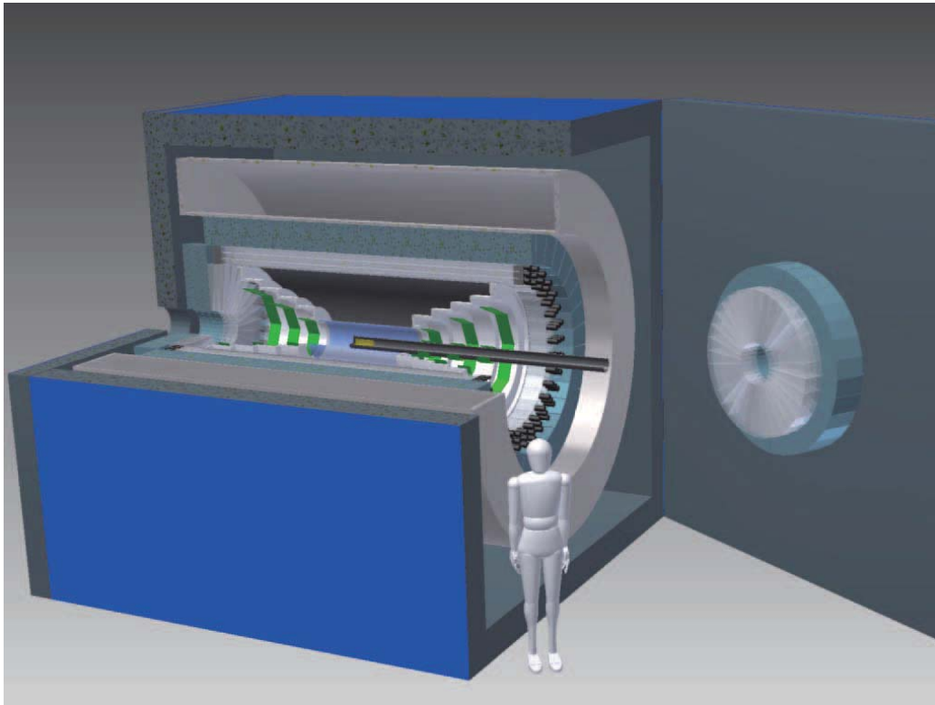
Figure 3: Conceptual design of the new CDS.
